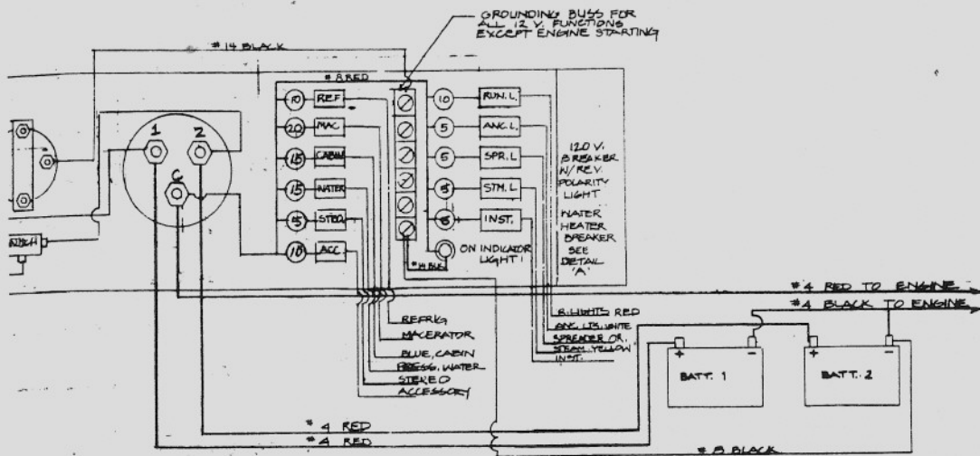
BACK VIEW OF MASTER PANEL WIRING DIAGRAM
