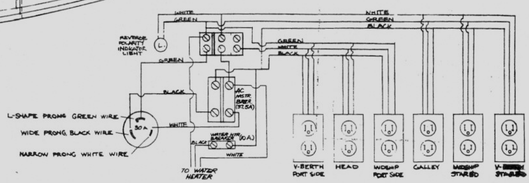
DETAIL A- 110 V. WIRING SCHEMATIC
