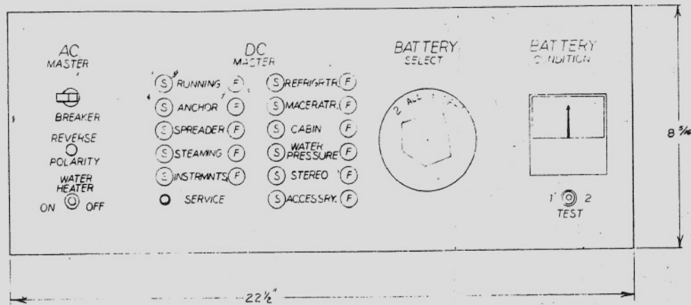
FRONT VIEW (1/2 SCALE)
