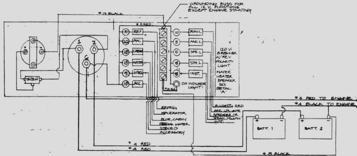
BACK VIEW OF MASTER PANEL WIRING DIAGRAM
